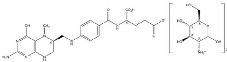
Figure 1: Chemical structure of 5-MTHF Glucosamine Salt
